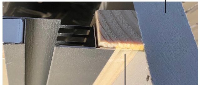
[With 3/4" Cedar Channel & Starter Strip]
