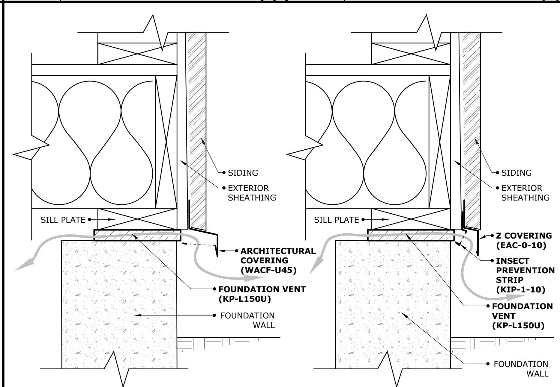
SCALE 3" = 1' COVERING DETAIL 5
